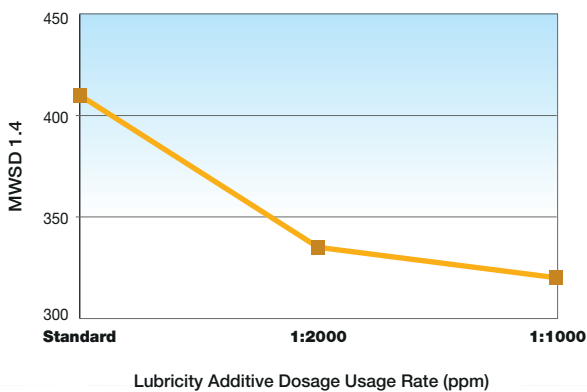
AR6900-D MAX - Friction Test Results
