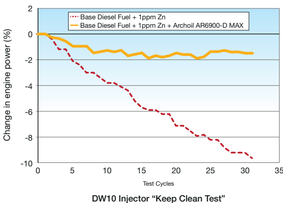
AR6900-D MAX - Maintenance Clean
