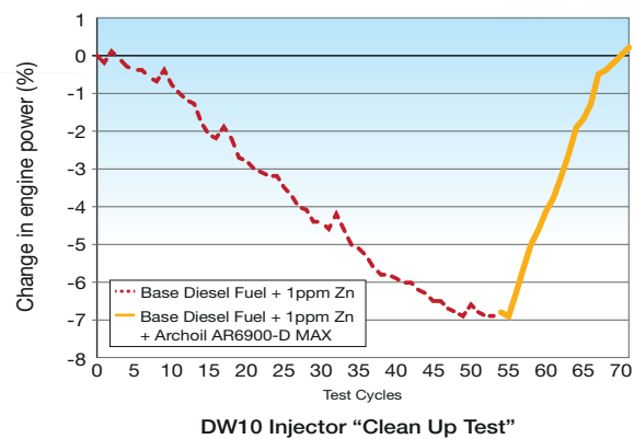
AR6900-D MAX - Clean Up Cycle
